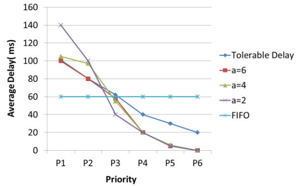
Fig. 3. The Average Delay time for Multiple SNs with Different Maximum Tolerable Delay.
